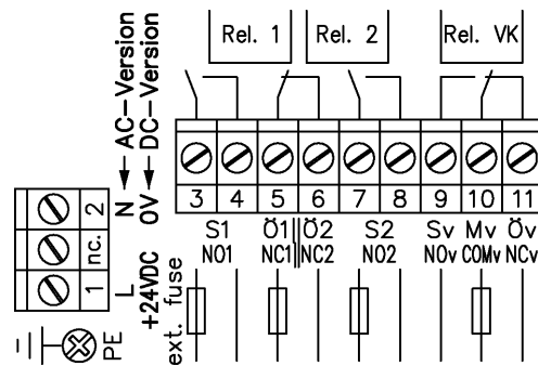
Fig.: 4.8: Connection diagram CPV1037
